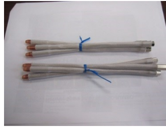
Part Number # 77700603 Three .035" Liner Complete Part Number # 77700604 Three .045" Liner Complete
