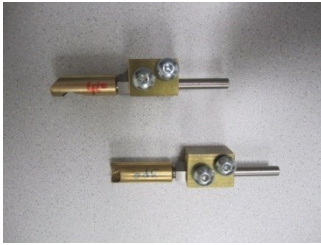
Part Number # 77700685 One 42 Deg Tip Holder for PIPE Part Number # 77700686 One 39 Deg Tip Holder for PLATE
